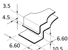
Dimensions mm
