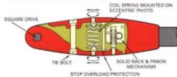
The working principle of Torqueleader Dial Measuring Torque Wrenches
