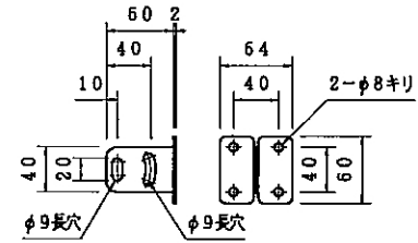
5 裏板金具 (S=1/5)
