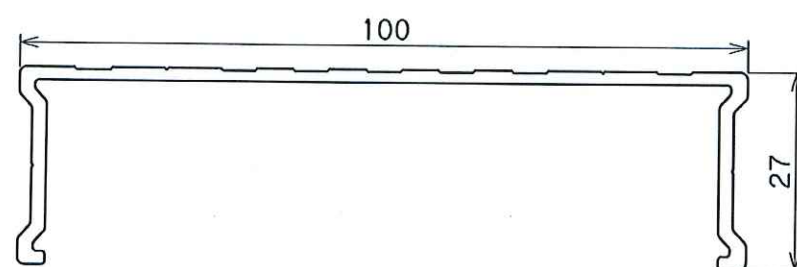
昇降面支柱 (1/1)
