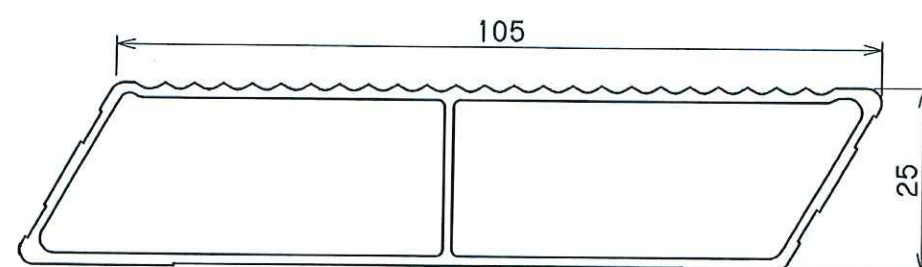
踏ざん (1/1)
