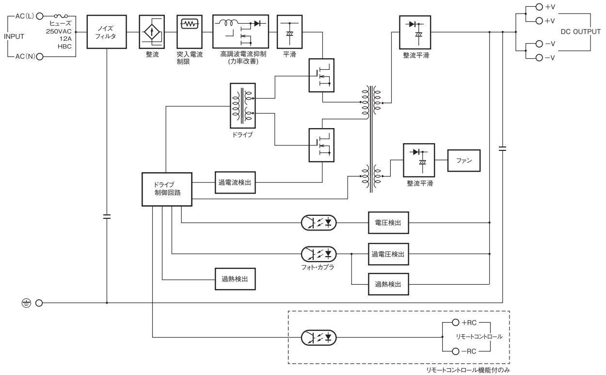
形S8FS-G600□□□ (600W)
