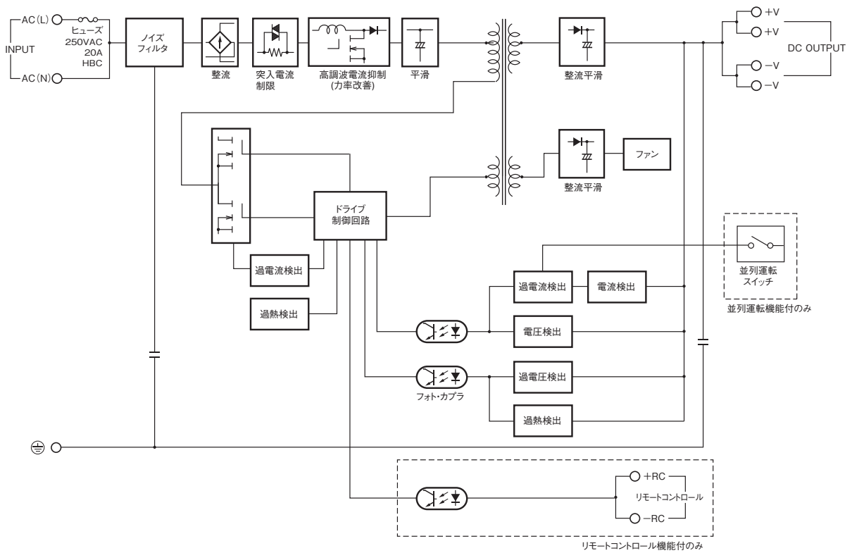
形S8FS-G600□□□ (600W)
